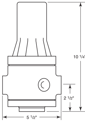
1" Socket or Threaded
