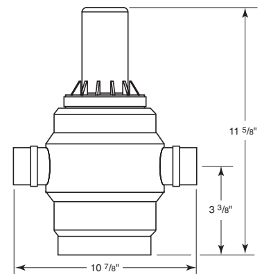
2" Spigot
