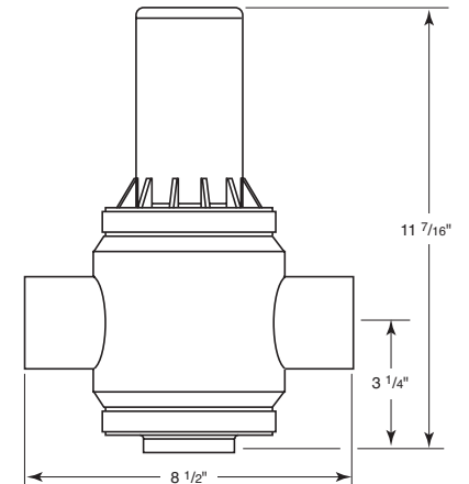
1 1/2" Spigot
